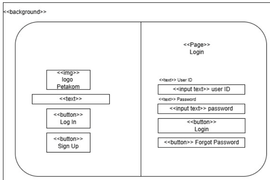
Figure 7.3 Login Page
