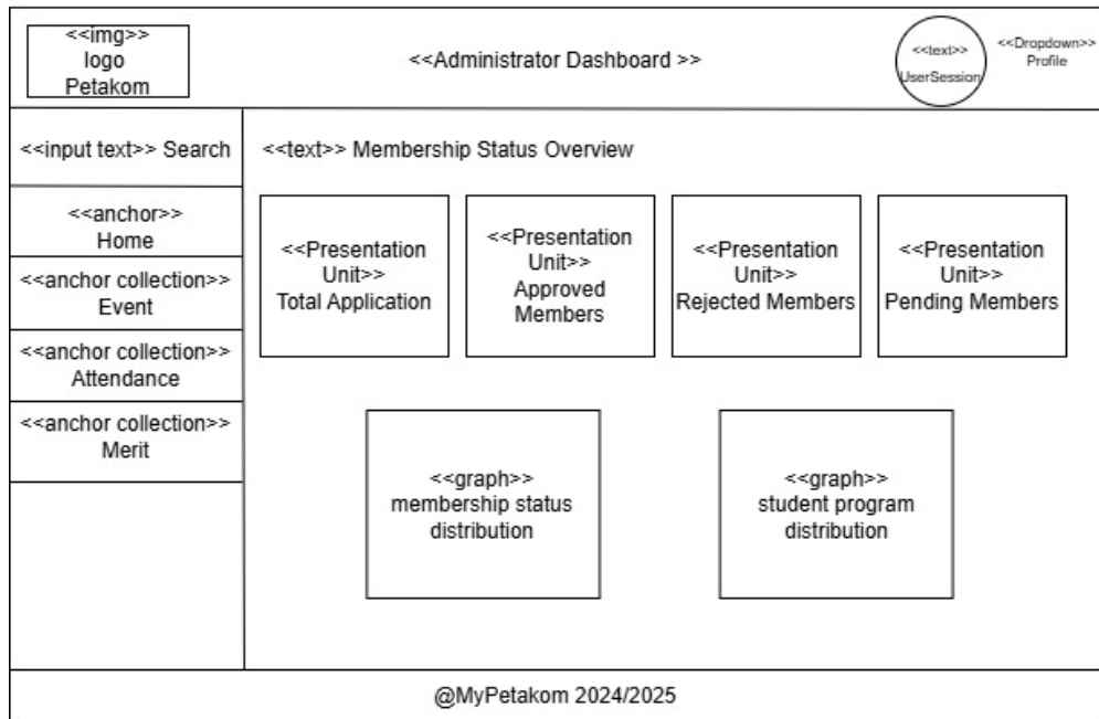
Figure 7.9 Administrator Dashboard
