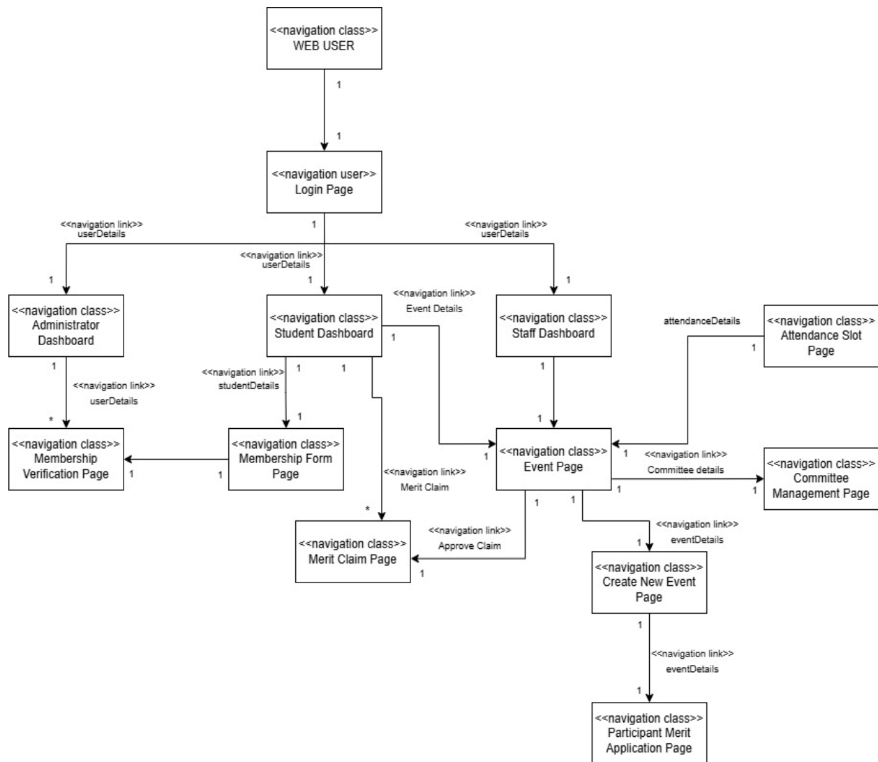
Figure 5.2 Hypertext Model
